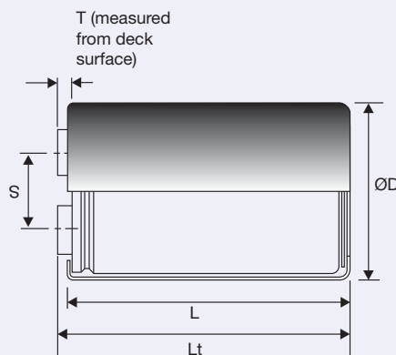
ALS36 Clamp Mounting
